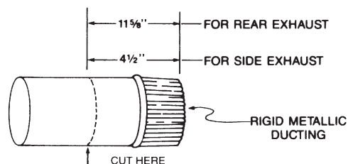
EXTENSION DUCT
